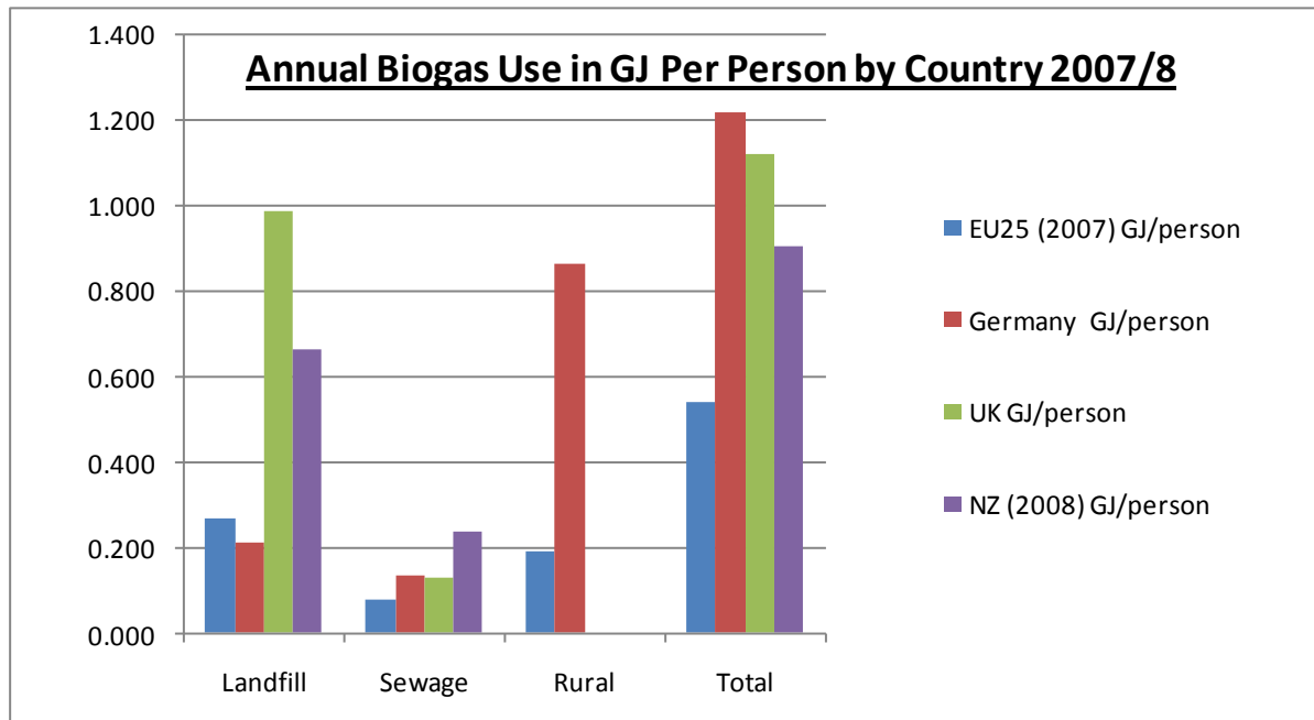
Figure 2. Relative per capita biogas utilisation in New Zealand and Europe, by gas source.
