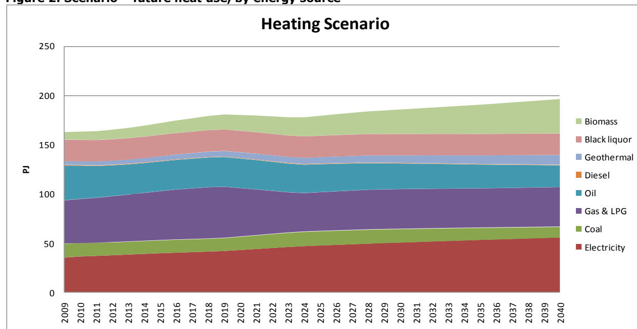
Total heat use from MED options study Mix based on an interpretation by East Harbour Energy
